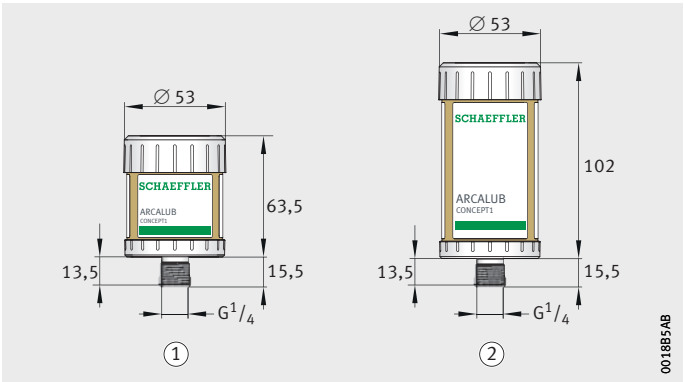
Figure 2 Dimensions
