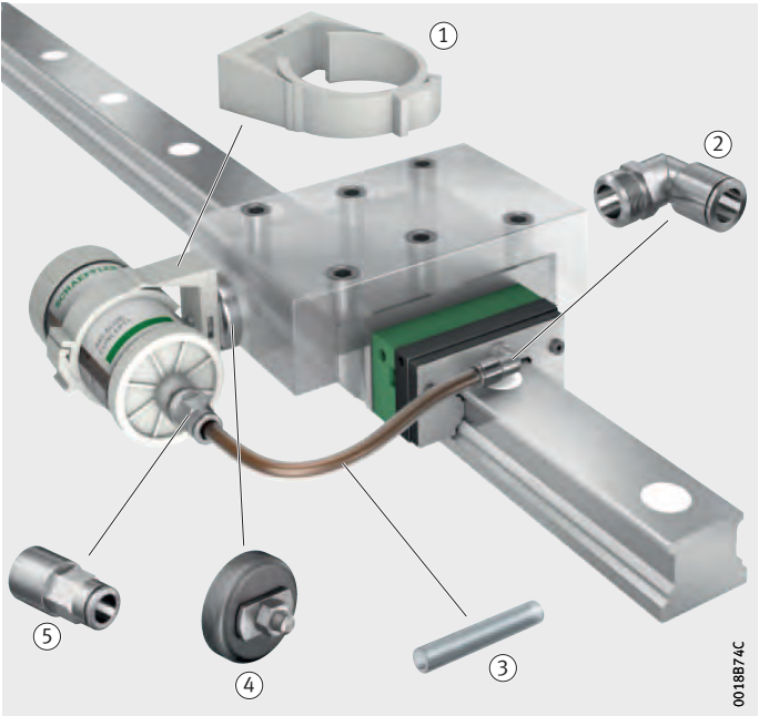
Figure 9 Lubrication of a linear guidance system
